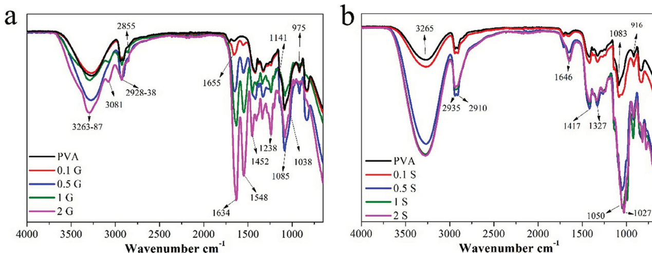
Figure 3. FTIR spectra of a) PVA/gelatin samples and b) PVA/sucrose samples 4000–650 cm -1 .
